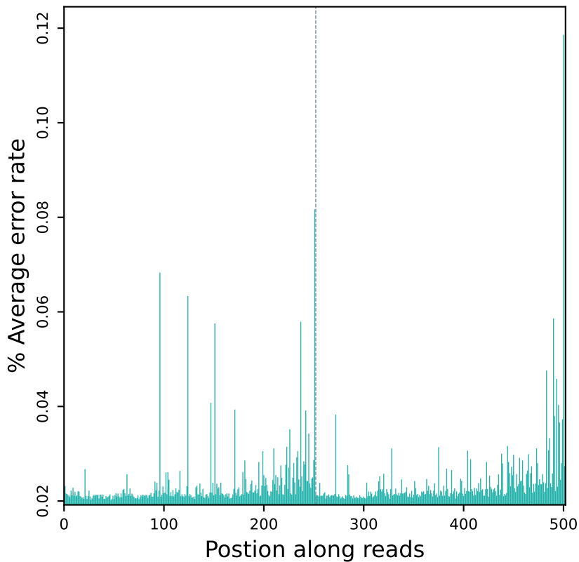
Error rate distribution along reads (R10703)
